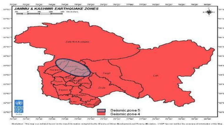
Figure 3.1 Seismic hazard map for Jammu & Kashmir State
