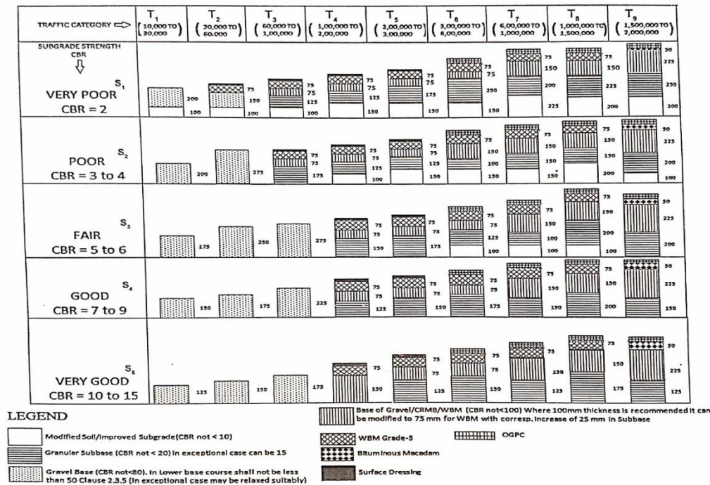
Figure 3: Pavement composition
